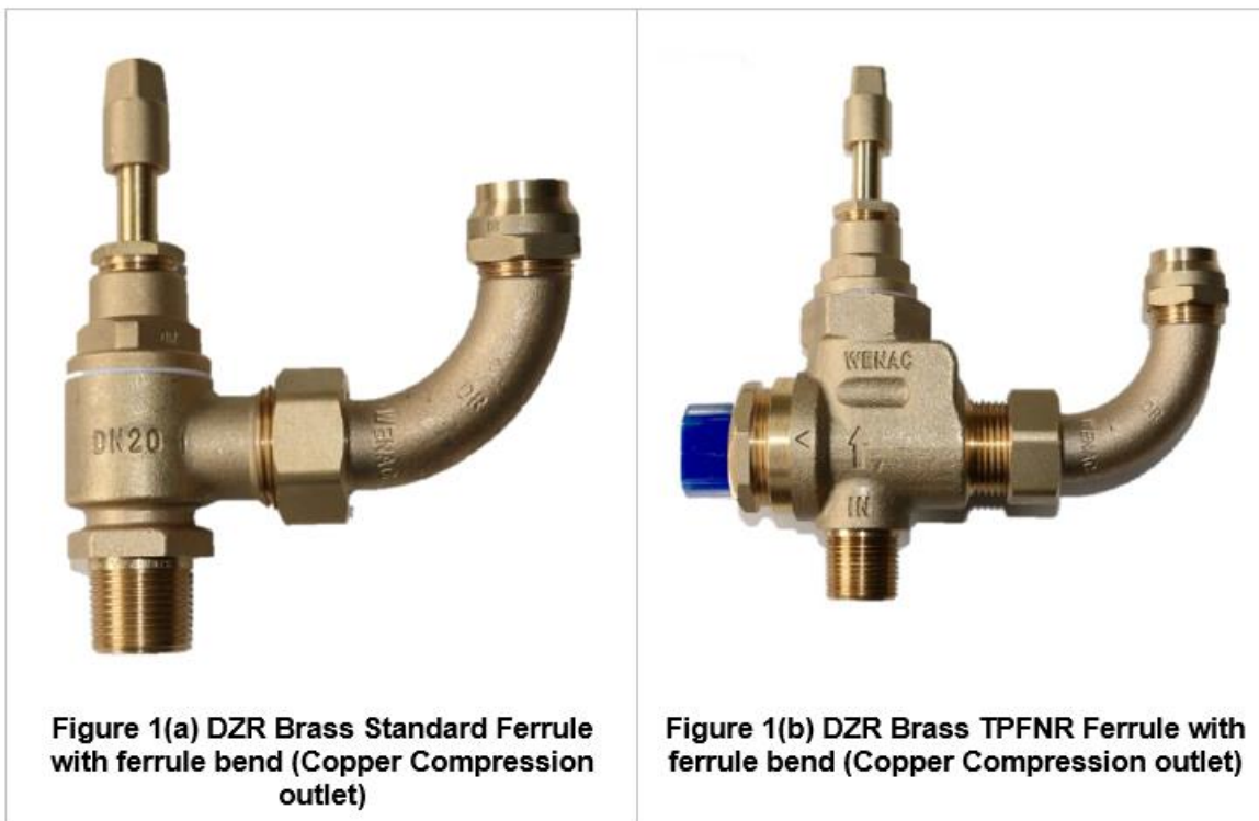
Figure 1: Standard and TPFNR ferrules with ferrule bends
