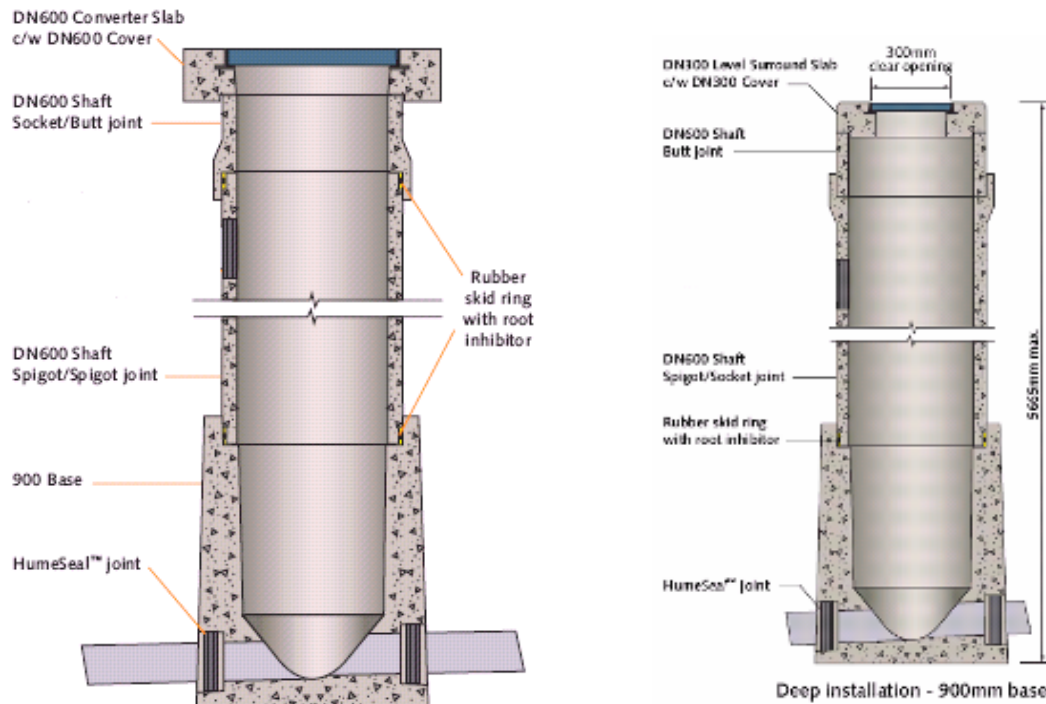
Figure 2 Humes™ Quicktee™ DN 600 Precast Maintenance Shaft with DN 600 / 300 access cover and frame
